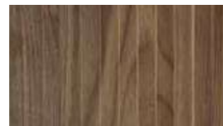
Matrix B
