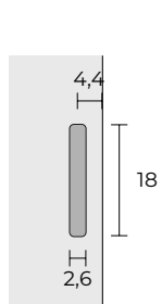
maniglia incassata Levia Levia built-in handle
