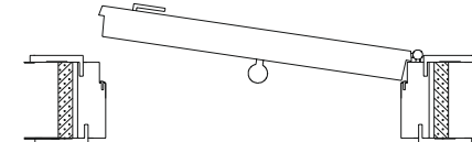
Portoncino / Entrance NTCPKVR
