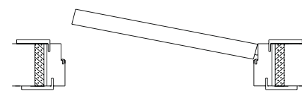
Cerniere a scomparsa / Concealed hinges NTCPKVR
